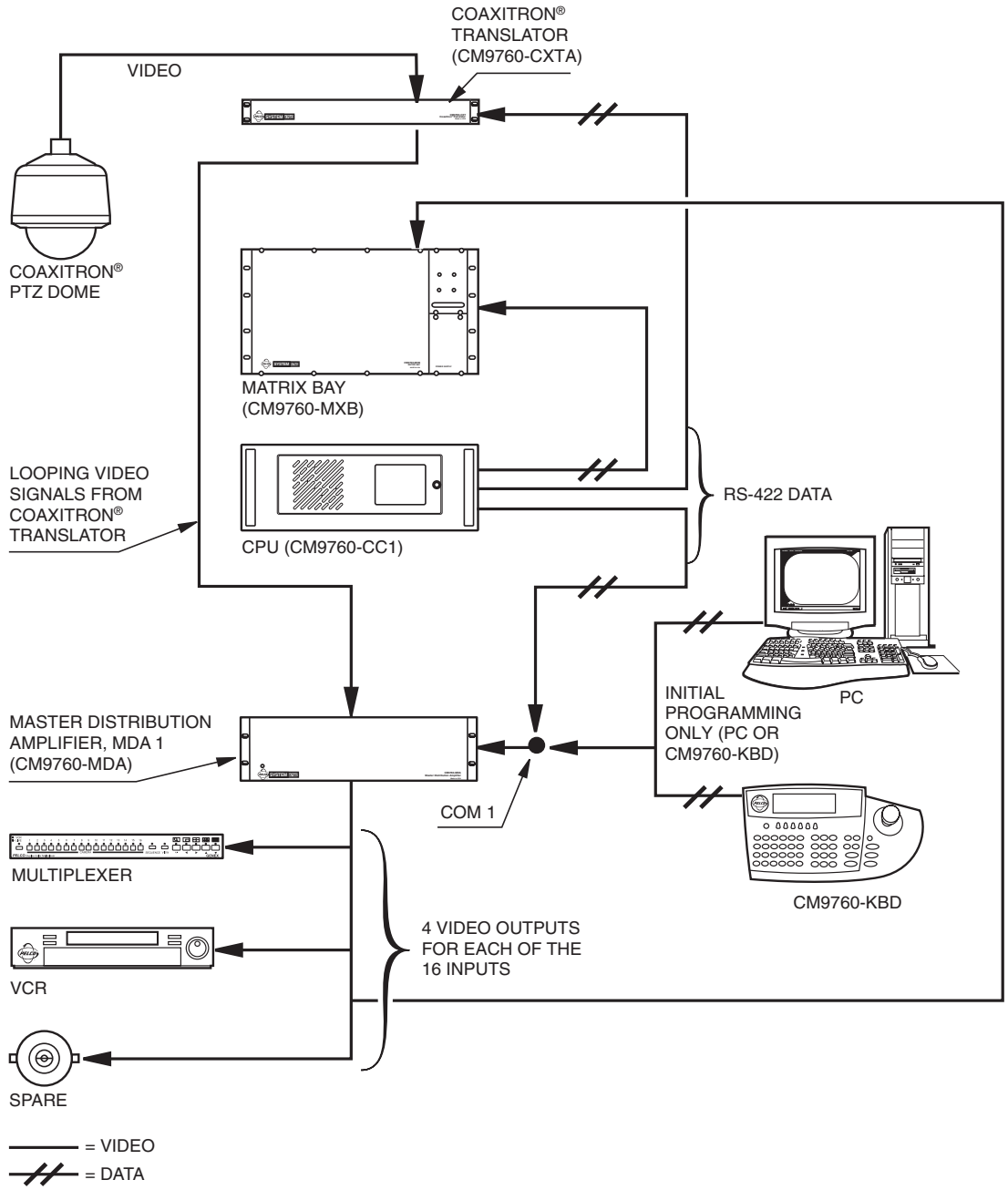
Figure 45. Coaxitron with System 9760 Setup
